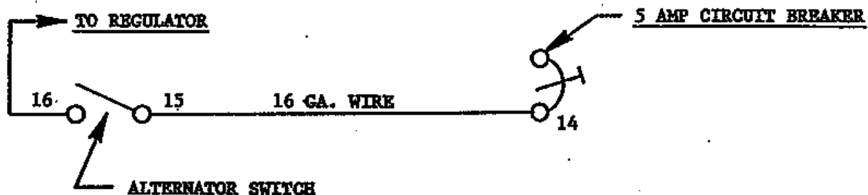
ELECTRICAL SYSTEM SCHEMATIC
